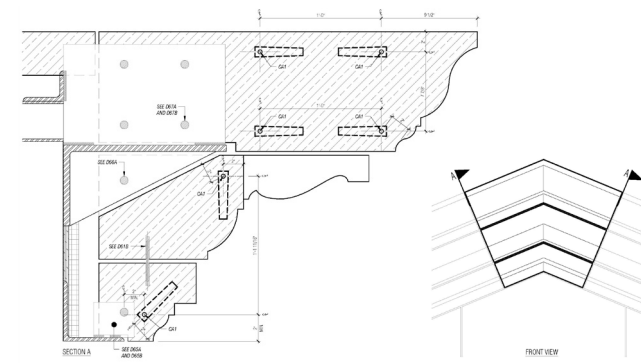
PICCO Group developed 205 pages of bespoke connection details. This section view shows one example of how the stone was anchored and braced with plates and pins to resist tipping out.
