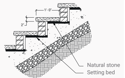
DIAGRAM OF TREAD INSTALLATION
